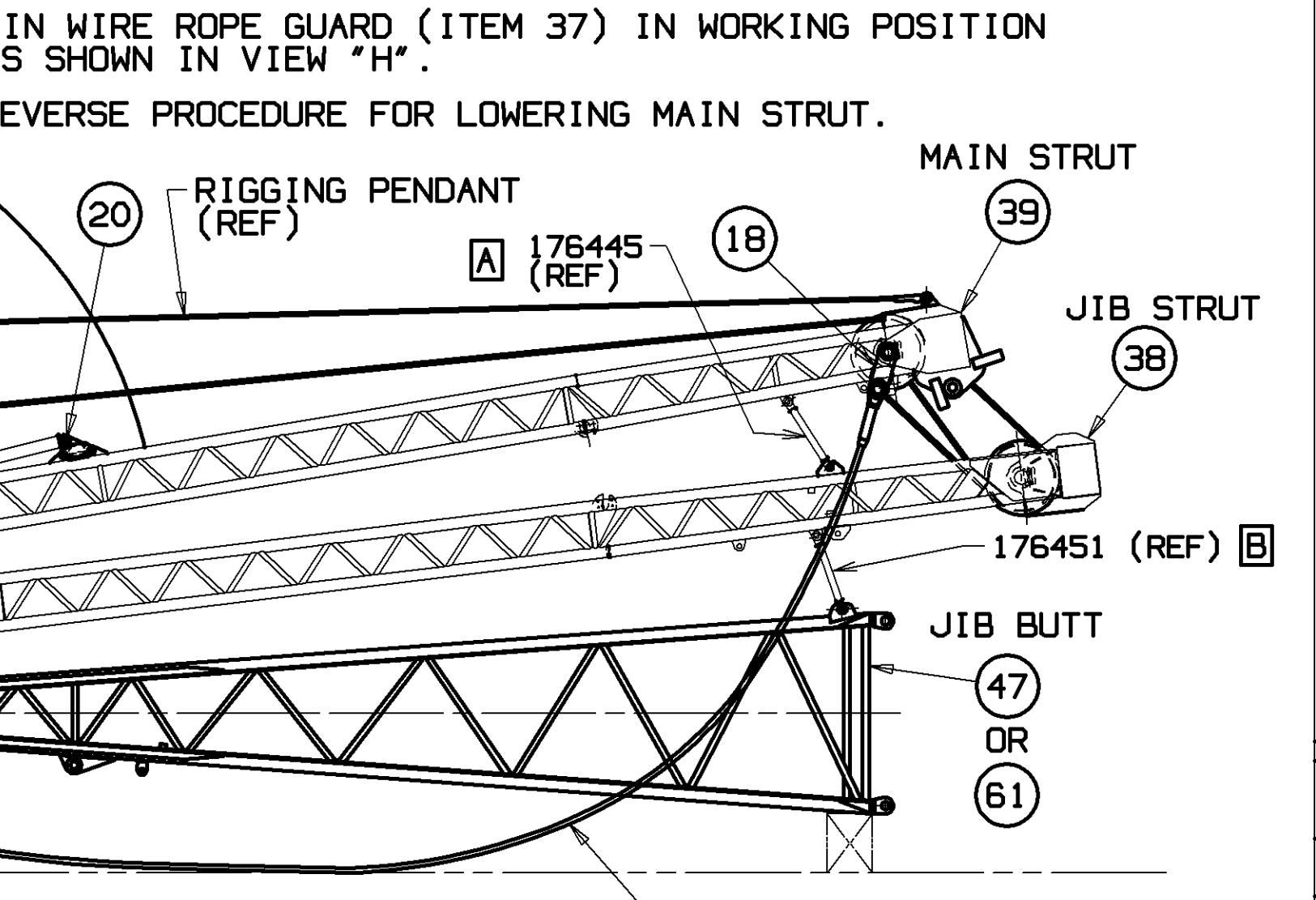
MAIN STRUT ERECTION
