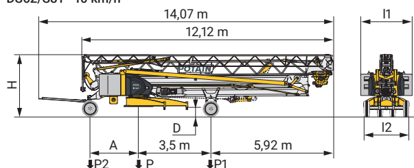
DS62/S81 - 10 km/h
