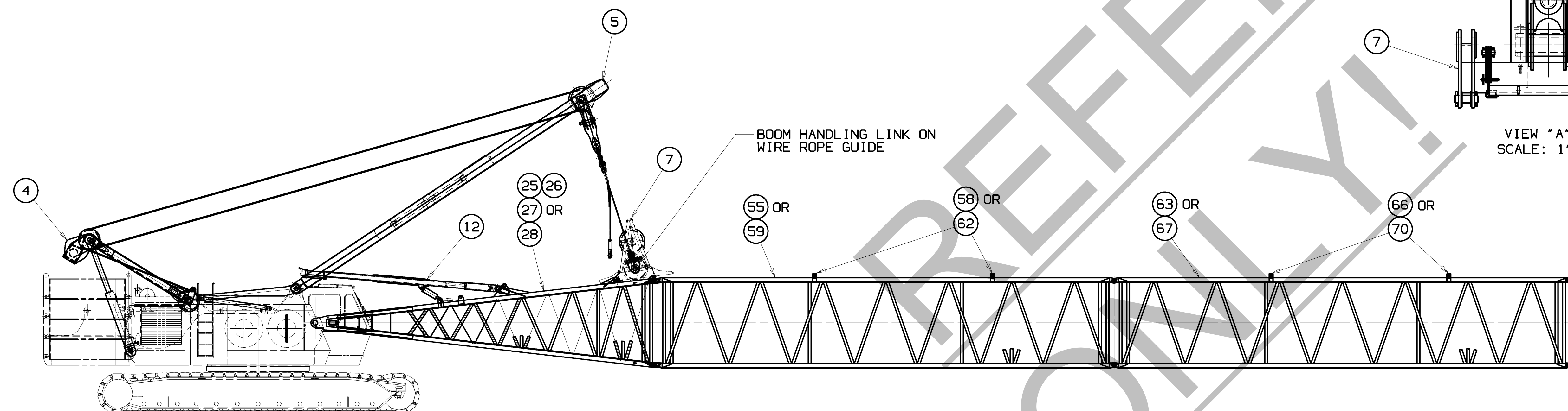
BOOM HANDLING WITH MAST
