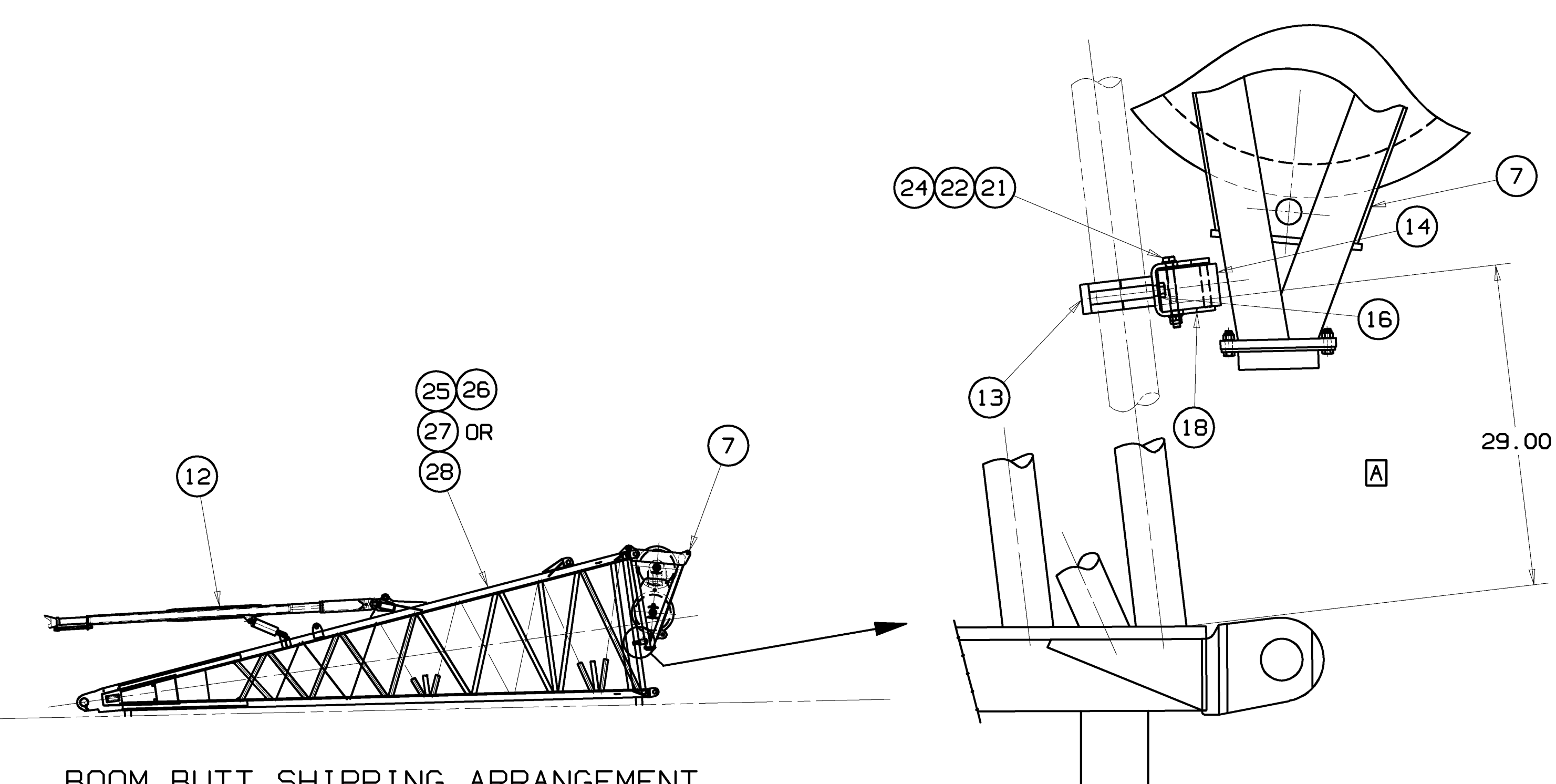
BOOM BUTT SHIPPING ARRANGEMENT
