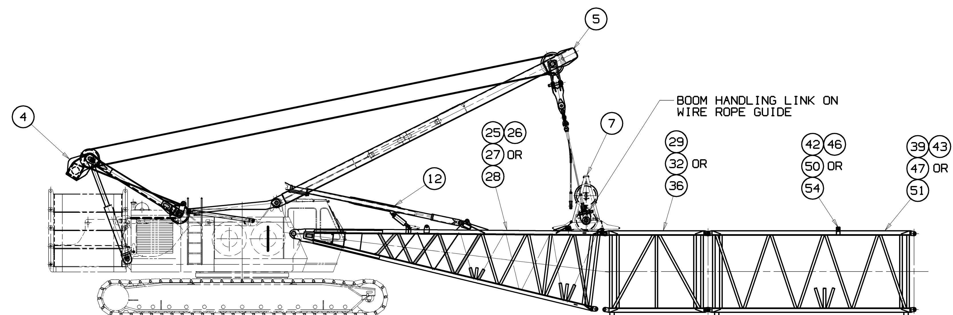
BOOM ASSEMBLY WITH MAST
