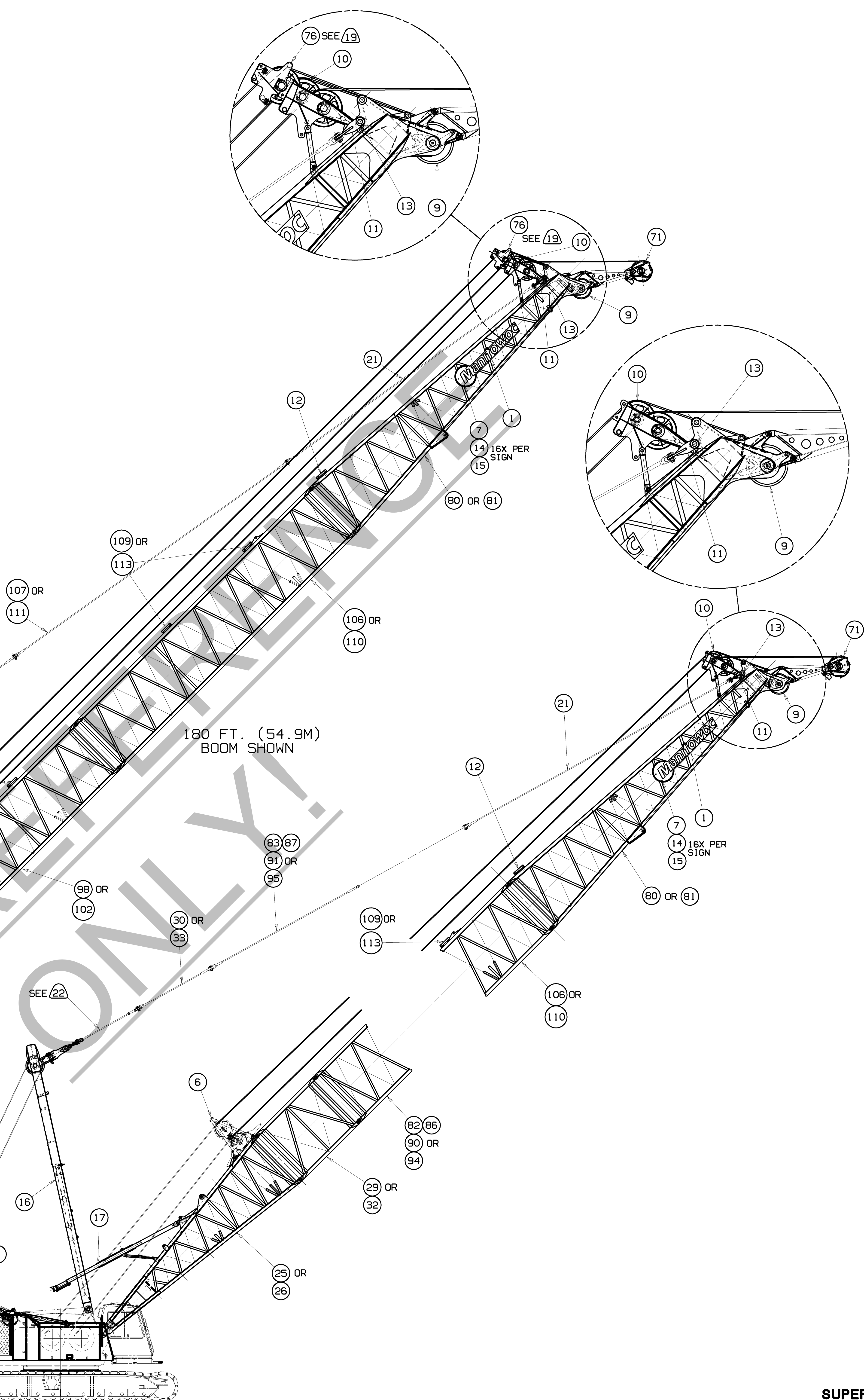
#22EL BOOM ASSEMBLY WITH NON-STOWABLE PENDANTS
