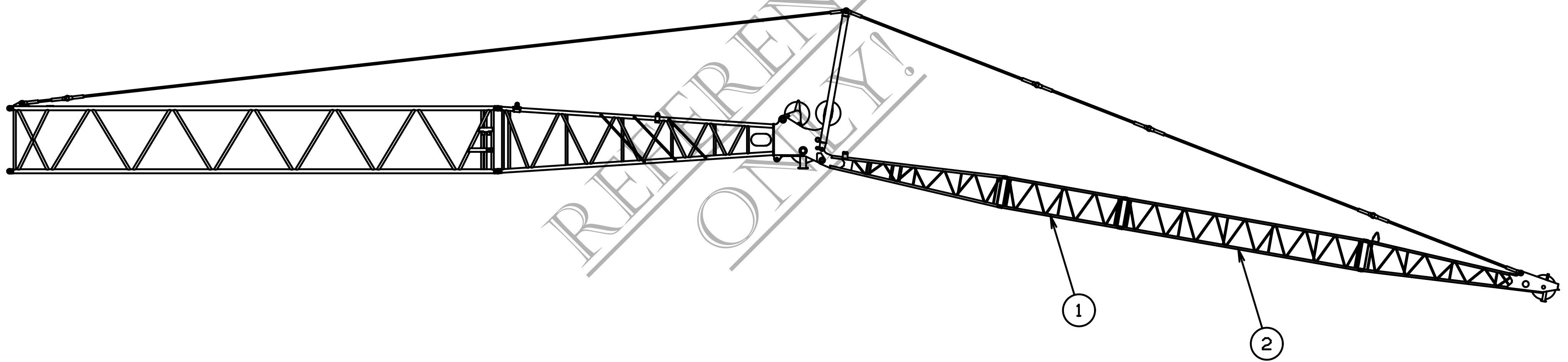
60 FT (18.3M) JIB SHOWN
