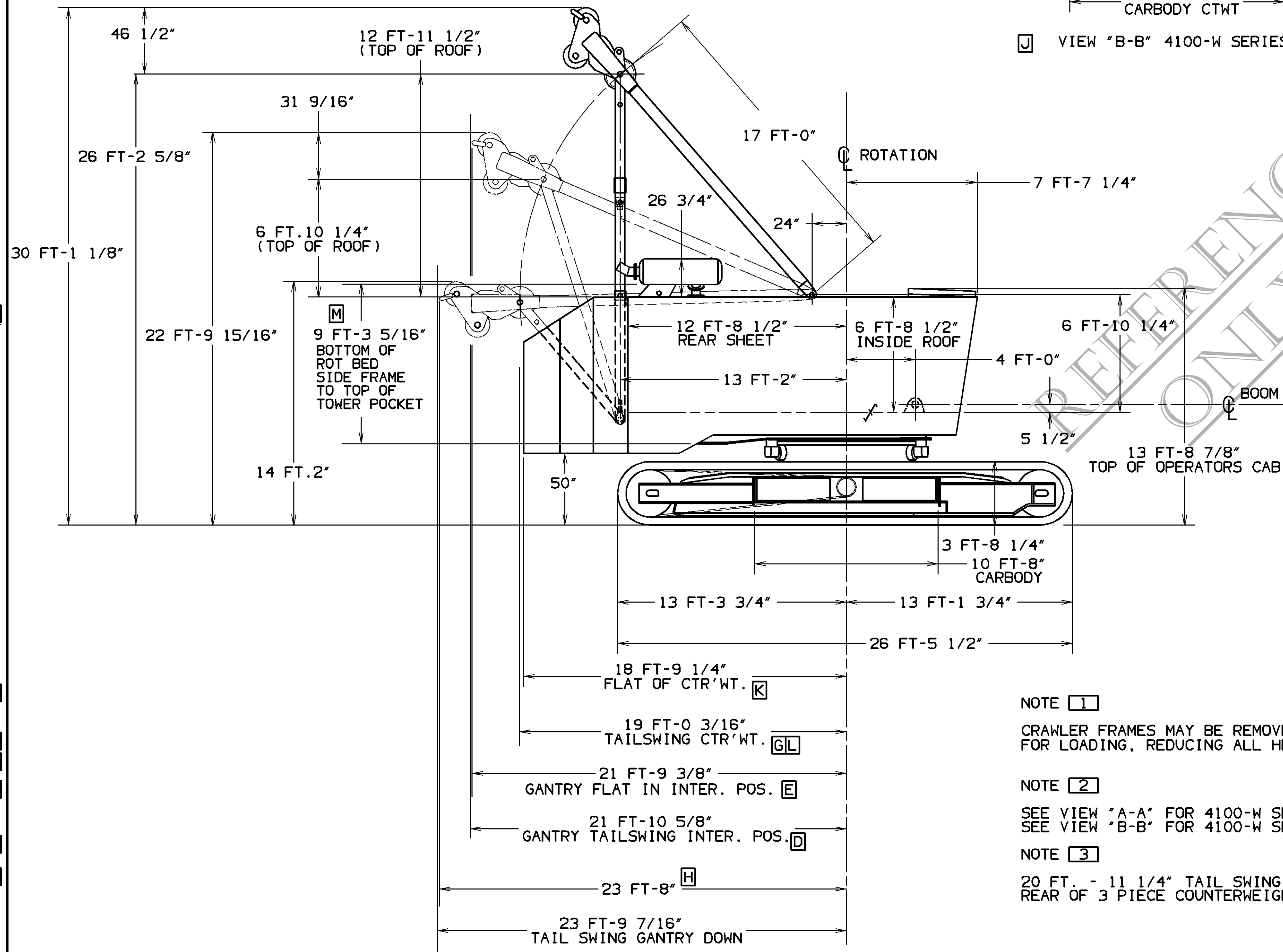
VIEW "A-A" 4100-W SERIES-1
