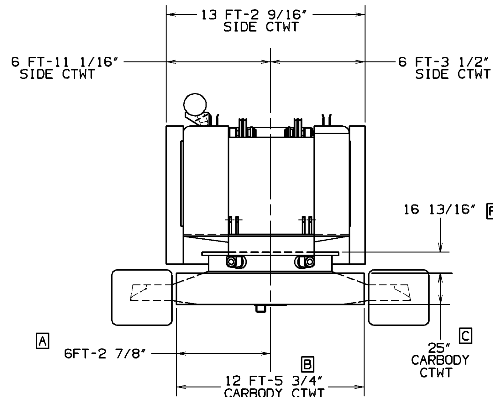
VIEW "B-B" 4100-W SERIES-2
