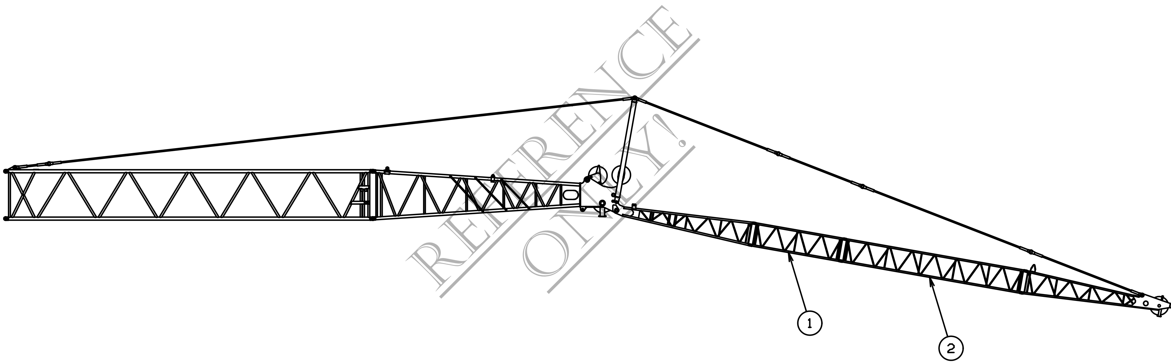
60 FT (18.3M) JIB SHOWN
