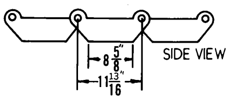
CRAWLER TREAD DETAILS
