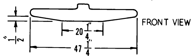
CRAWLER TREAD DETAILS
