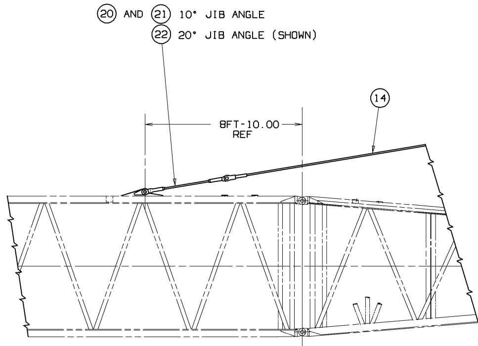
10° OR 20° JIB ANGLE
