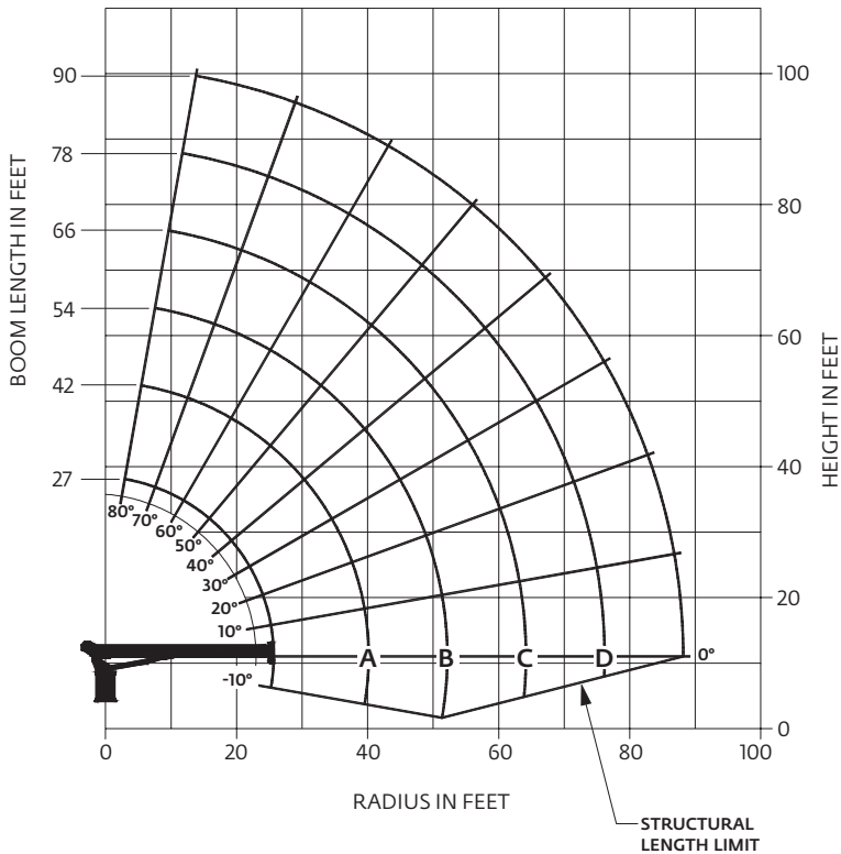
Load chart
