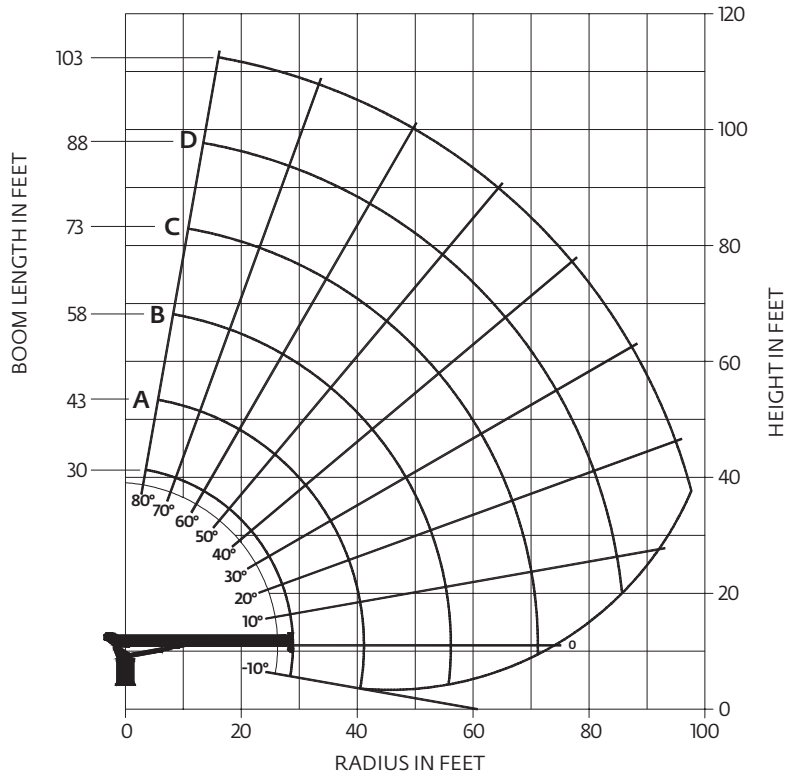
Load chart
