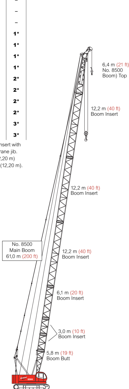
Model 8500 Main Boom 61,0 m (200 ft)
