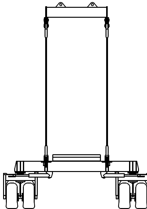
MAX-ER 225 On 2250 55,000 Lb. (24 950 kg) Wheeled Counterweight
