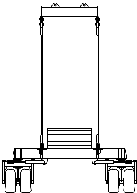
MAX-ER 225 On 2250 135,000 Lb. (61 230 kg) Wheeled Counterweight
