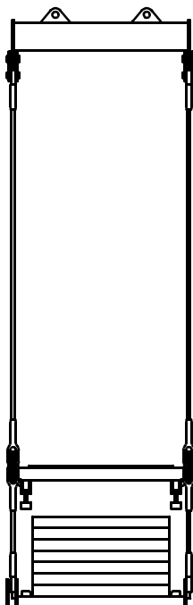
MAX-ER 225 On 2250 175,000 Lb. (79 380 kg) Hanging Counterweight
