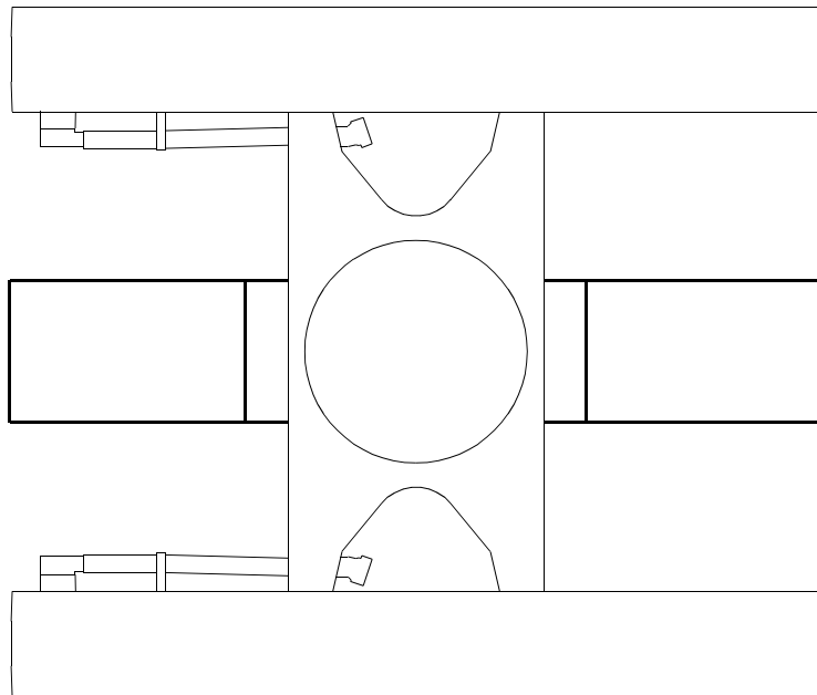
2250 SERIES 2 60,000 Lb. (27 220 kg) Carbody Counterweight
