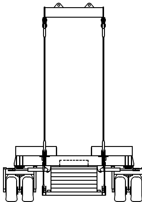
MAX-ER 225 On 2250 225,000 Lb. (102 060 kg) Wheeled Counterweight
