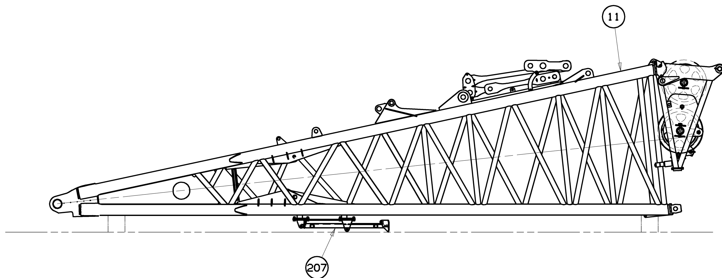
BOOM BUTT SHIPPING ARRANGEMENT SCALE 0.015
