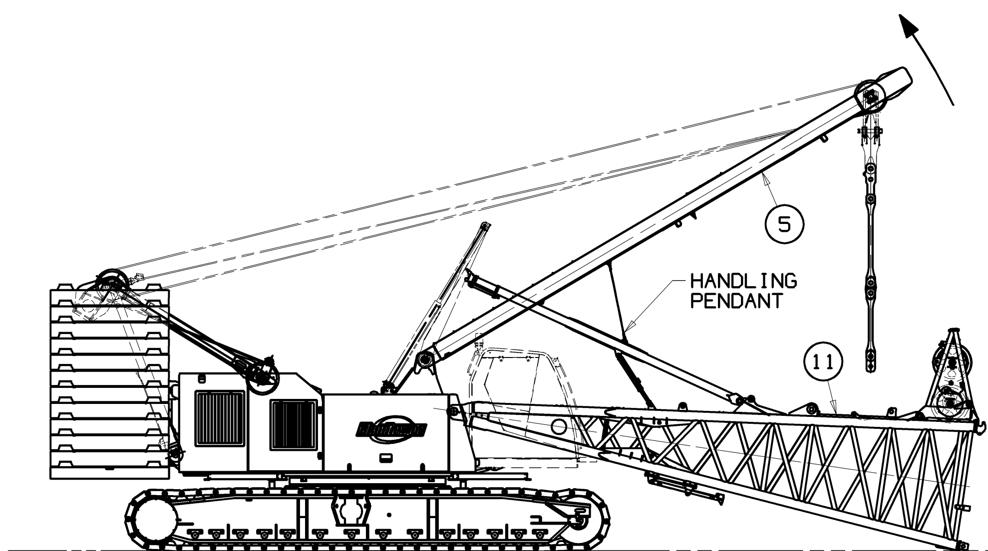
RAISING BOOM STOPS WITH MAST
