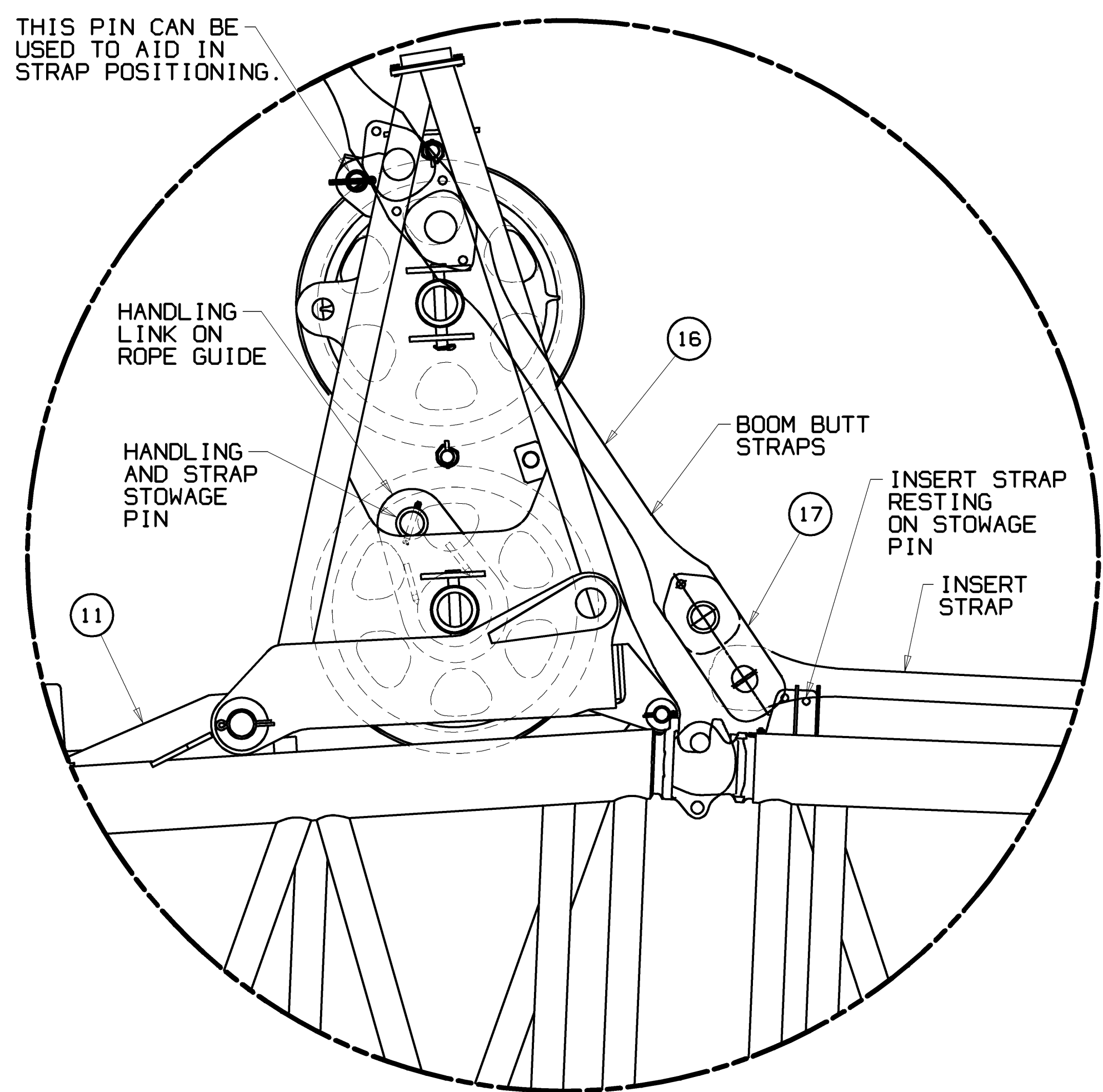
DETAIL "D" SCALE: 0.1
