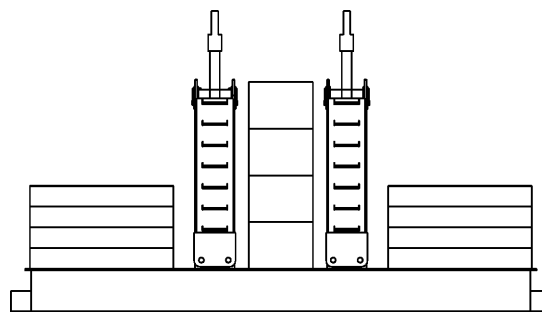
599,800 Lb. (272 060 kg) Hanging Counterweight 8 Side Boxes - 4 Center Boxes
