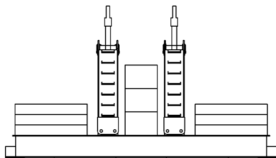
467,800 Lb. (212 190 kg) Hanging Counterweight 6 Side Boxes - 3 Center Boxes
