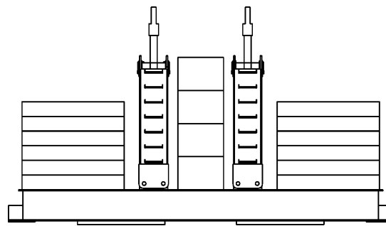
775,800 Lb. (351 900 kg) Hanging Counterweight 12 Side Boxes - 4 Center Boxes
