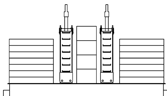
863,800 Lb. (391 810 kg) Hanging Counterweight 14 Side Boxes - 4 Center Boxes
