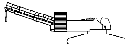
160.0 ft Boom, 230.0 ft Luffing Jib
