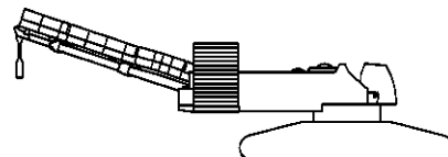
180.0 ft Boom, 310.0 ft Luffing Jib
