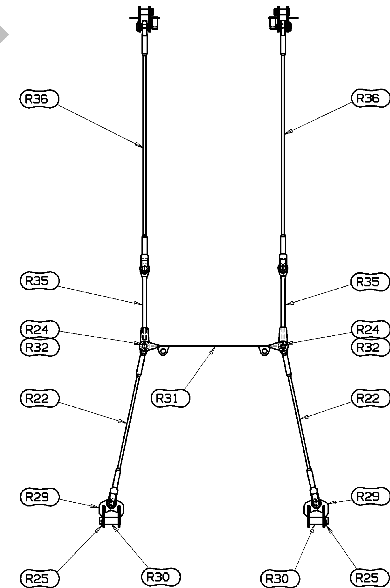
140 FT MAST - 380 FT & 440 FT BOOM SCALE 0.4=1FT
