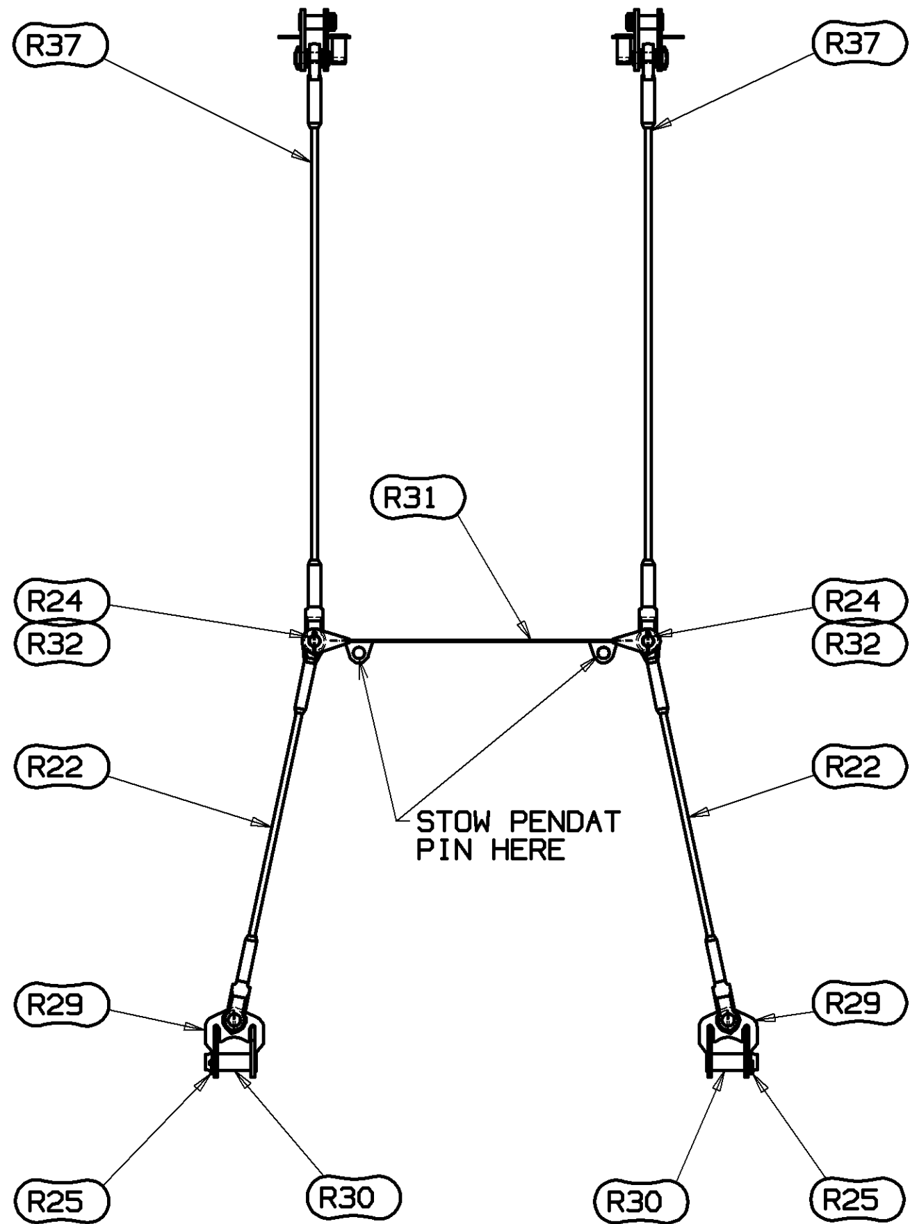
140 FT MAST - 400 FT BOOM SCALE 0.4=1FT
