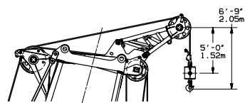
30 US TON (27 mTONNE) WEIGHT BALL TO JIB POINT MINIMUM DISTANCE #79A LUFFING JIB - 1 PART OF LINE MINIMUM DISTANCE MEASUREMENTS BASED ON 87° BOOM ANGLE AND 75° LUFFING JIB
