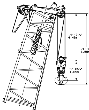
350 US TON (317.5 mTONNE) BLOCK TO JIB POINT MINIMUM DISTANCE #78A LUFFING JIB - 1 DRUM 18 PARTS OF LINE MINIMUM DISTANCE MEASUREMENTS BASED ON 87° BOOM ANGLE AND 75° LUFFING JIB
