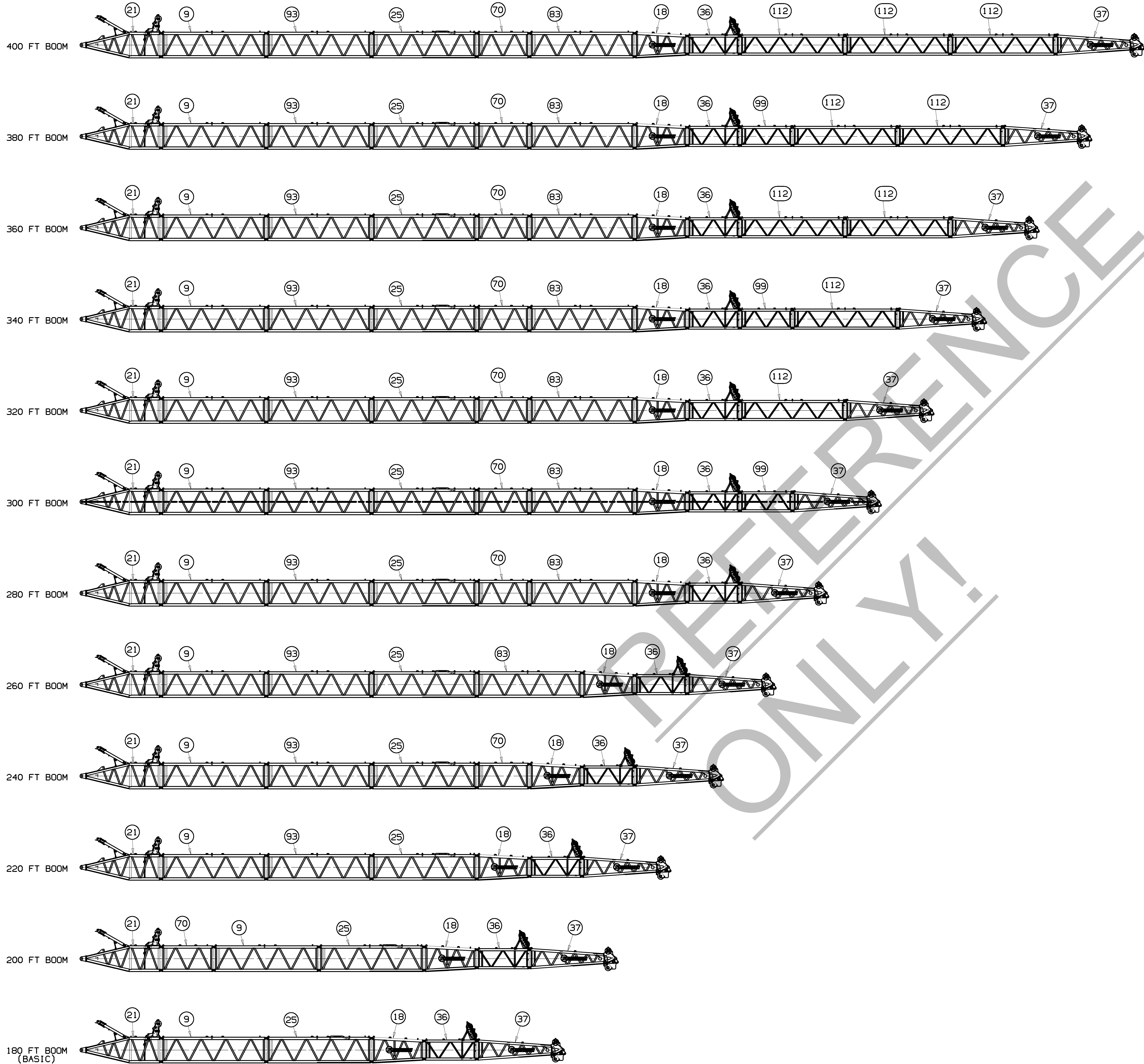
RECOMMENDED BOOM ASSEMBLY
