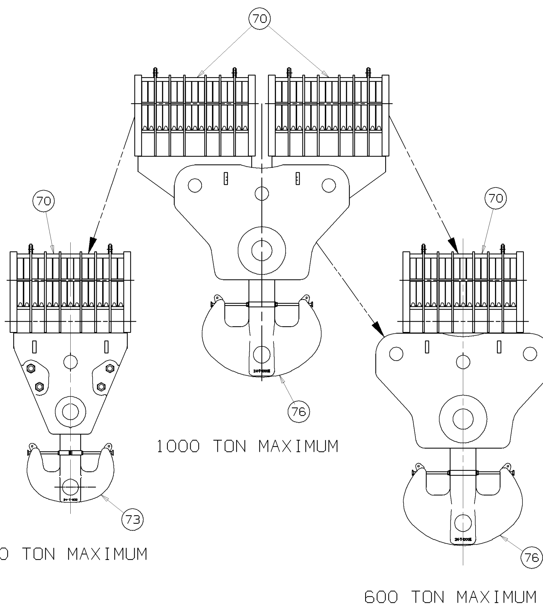
OPTIONAL BLOCK ASSEMBLY
