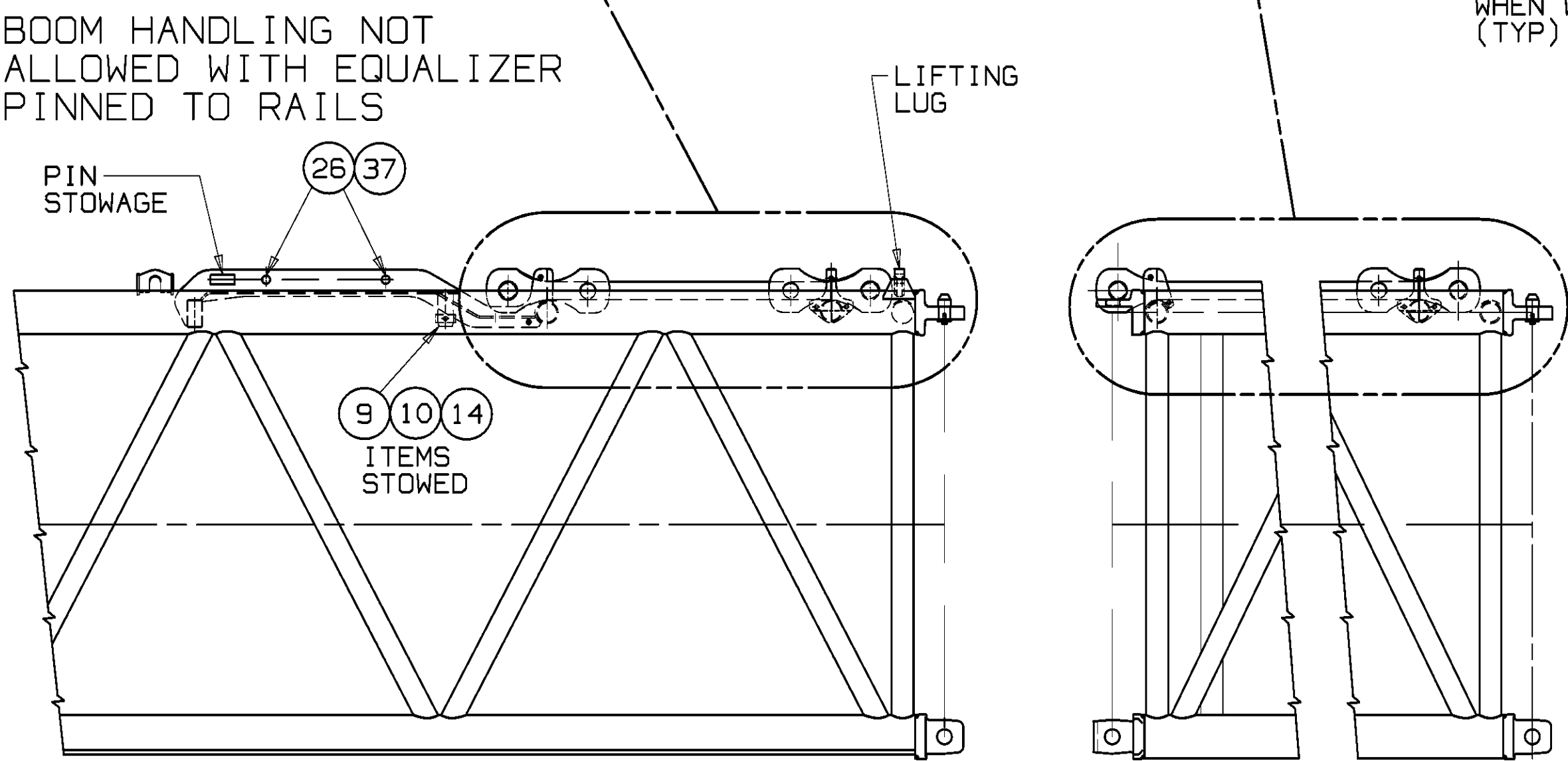
BOOM HANDLING NOT ALLOWED WITH EQUALIZER PINNED TO RAILS BOOM SUPPORT STRAP STOWAGE ON 40 FT INSERT WITH EQUALIZER RAILS.
