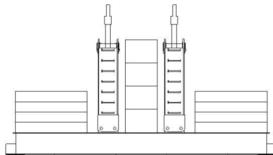
458,700 lb Crane Counterweight 24 Side Boxes
