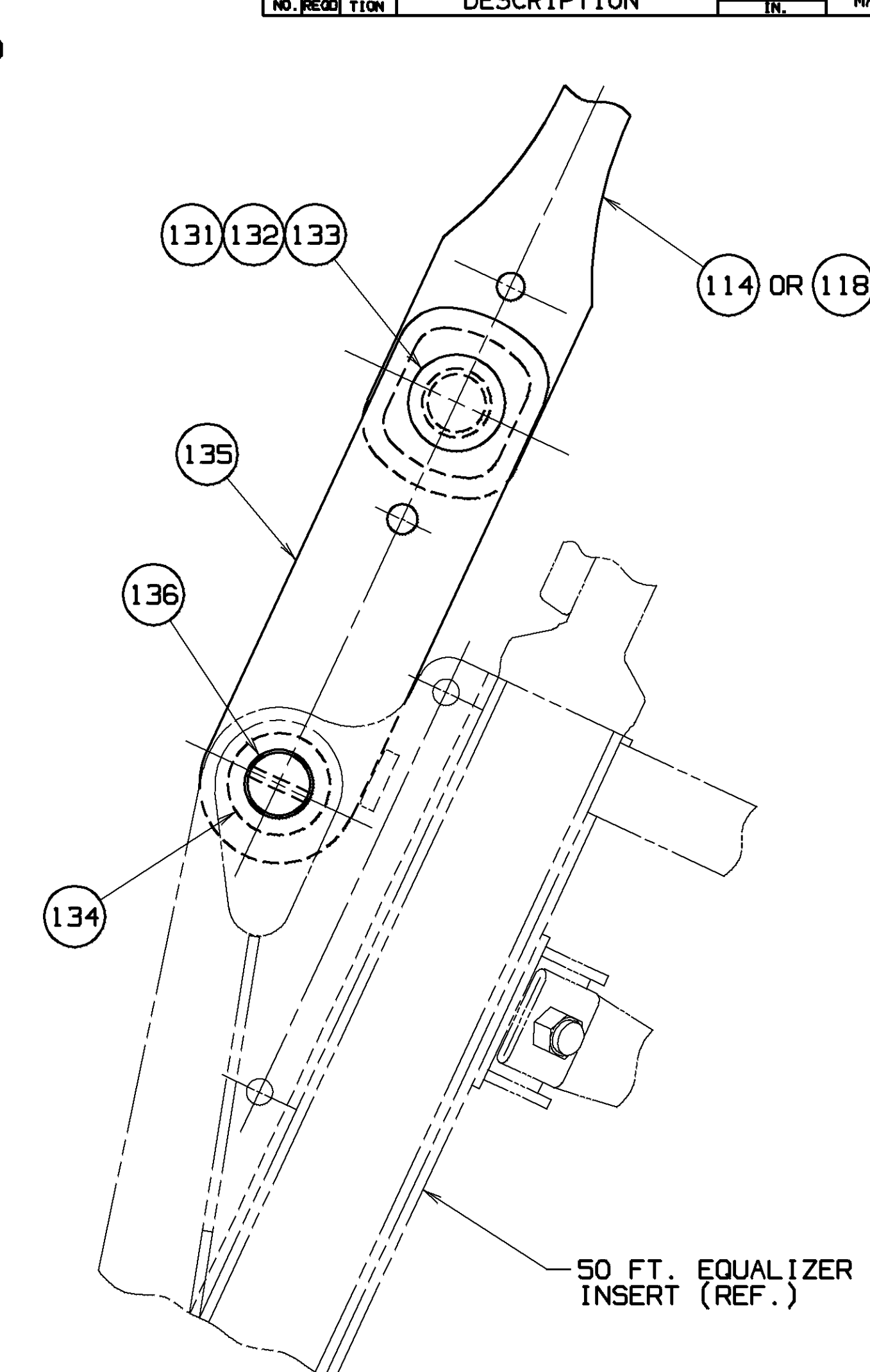
VIEW "D" - PINNING LOCATION FOR BOOM LENGTHS OF 275-375 FT. (83.8-114.3M) SCALE: 2=1FT.
