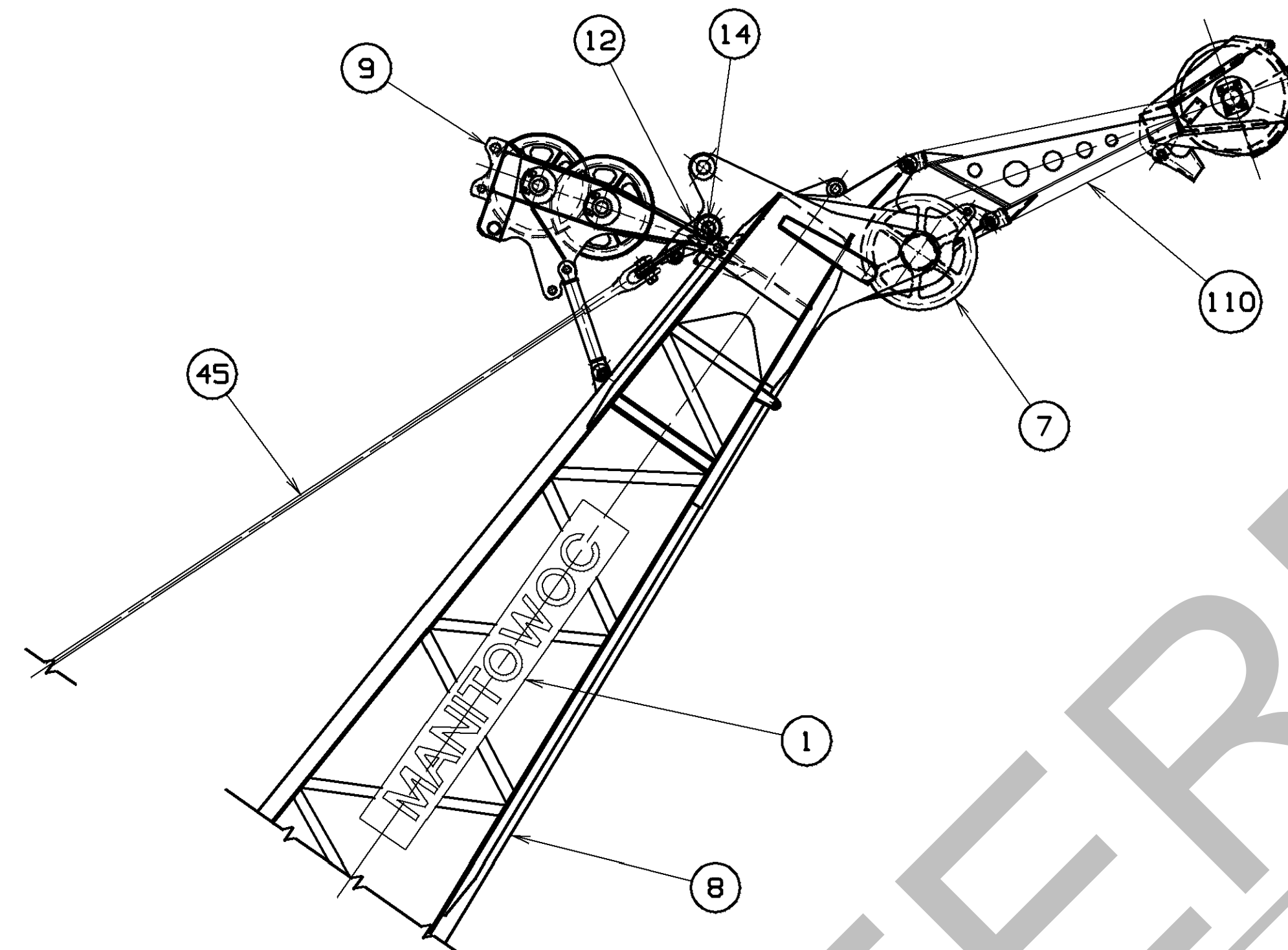
VIEW SHOWING OPTIONAL UPPER BOOM POINT ASSEMBLY (ITEM 109)
