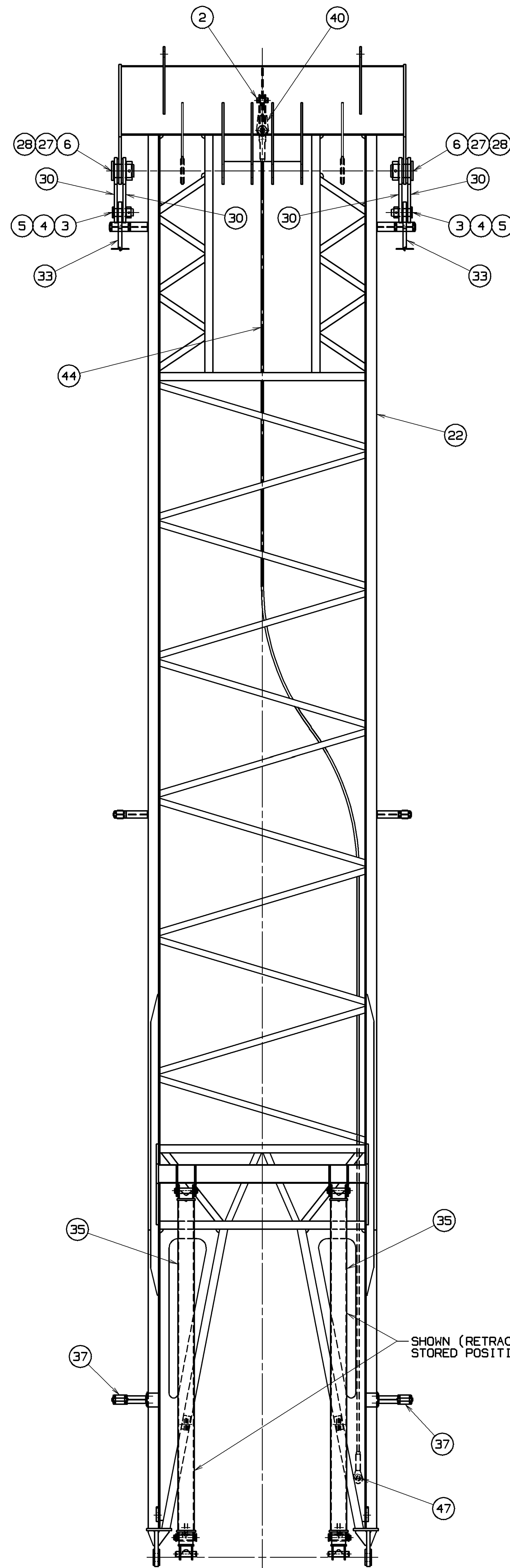
VIEW "E" - "E" SCALE: .50=1FT.
