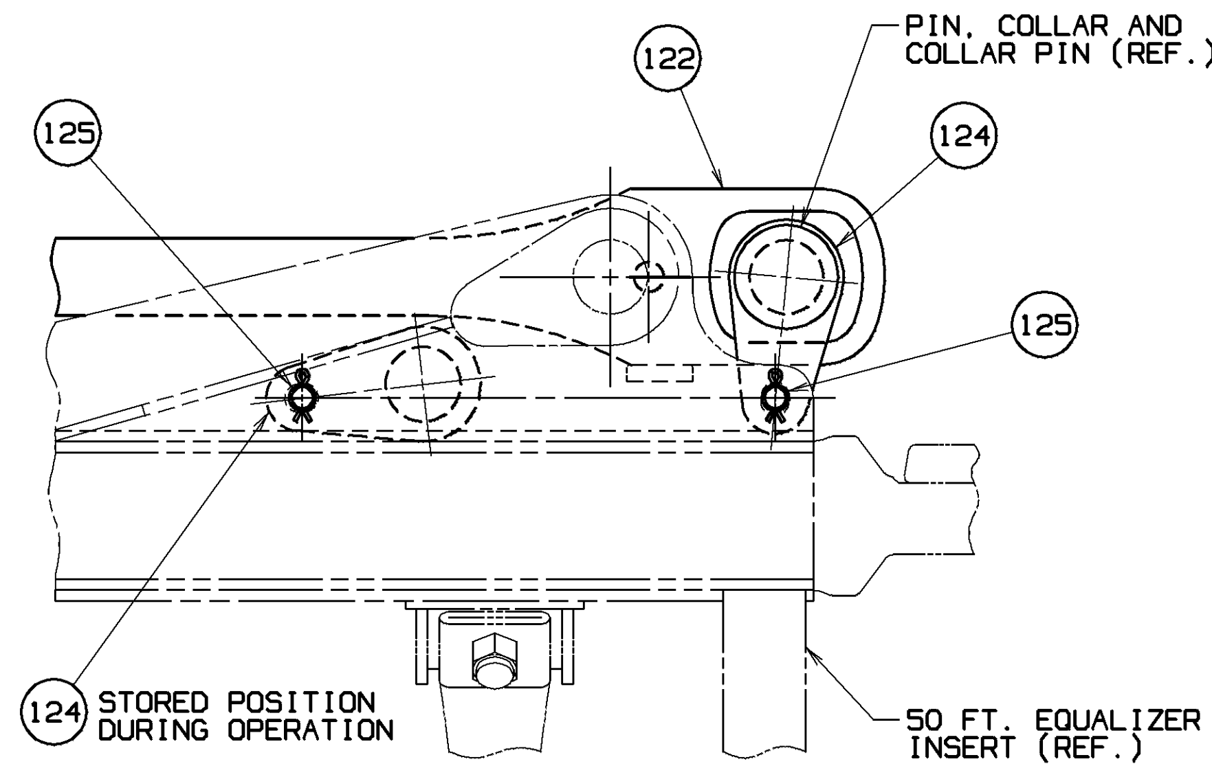
VIEW "C" - STORAGE OF STRAP ASSEMBLY 50 FT. (15.2M) USING LINKS (ITEM 124) FOR BOOM LENGTHS OF 175-250 FT. (53.3-76.2M) - SEE 19 SCALE: 2=1FT.
