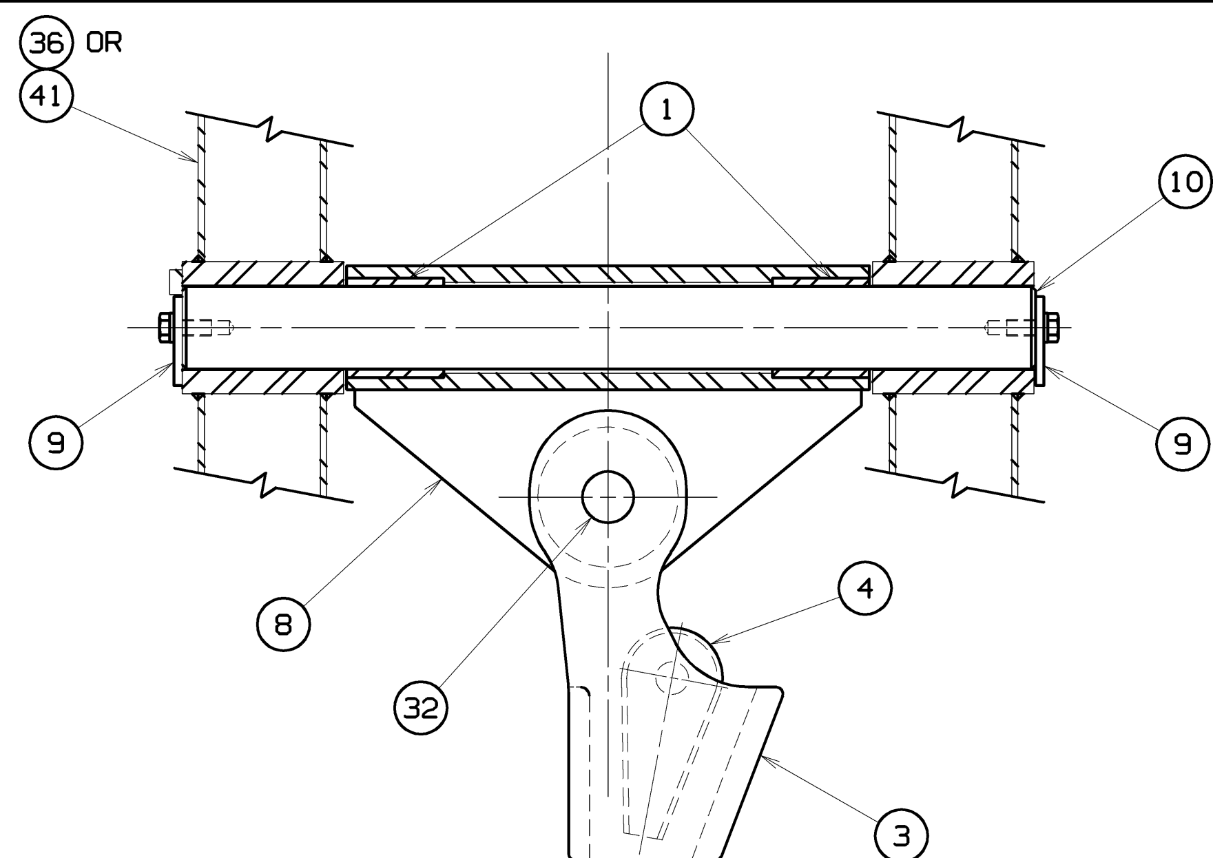
SECTION D-D SEE 3 SCALE: 3=1 FT.
