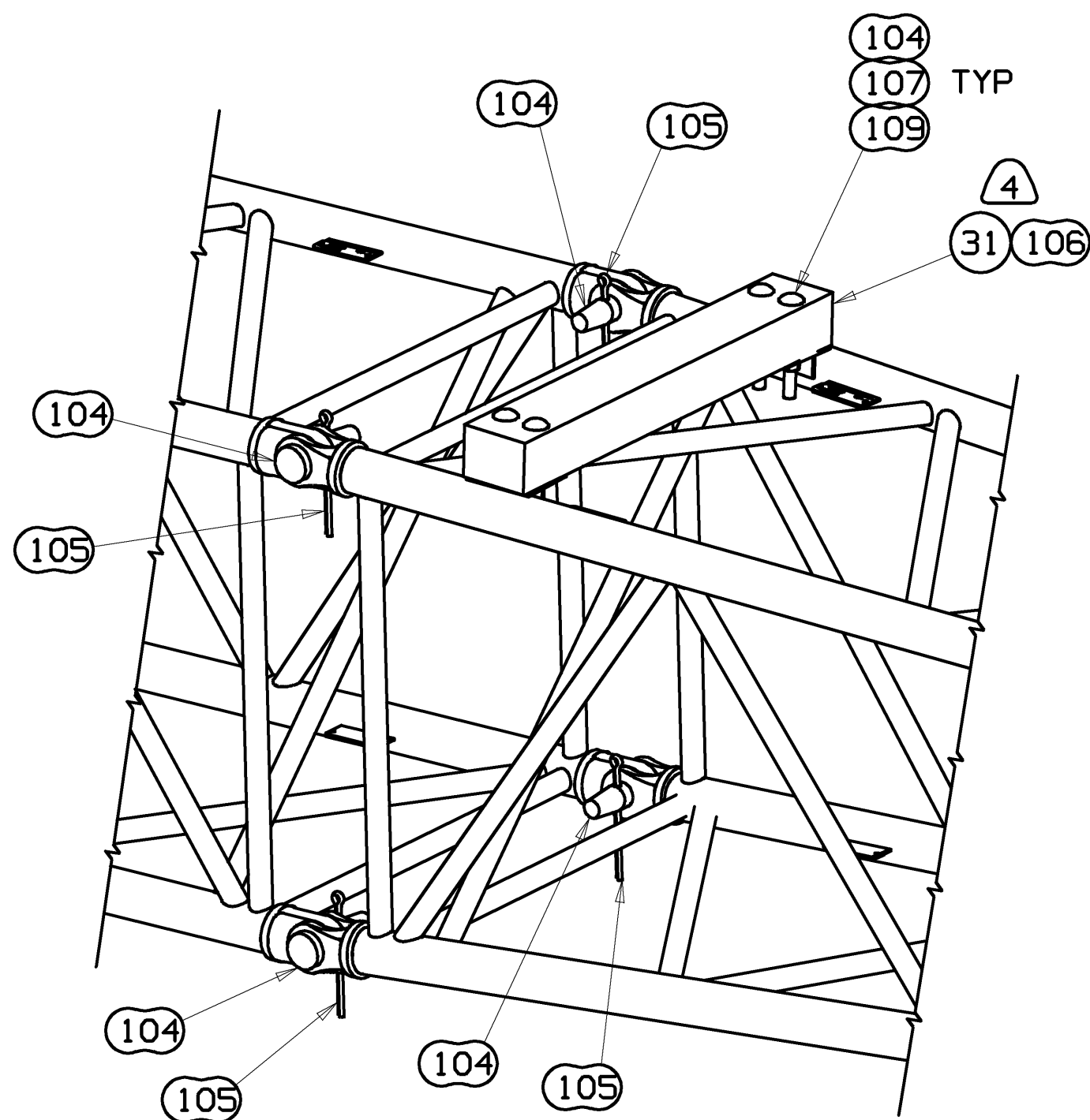
DETAIL J TYPICAL JIB JOINT PINS SCALE: 1.5=1FT
