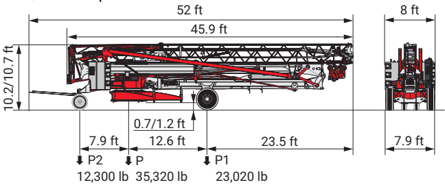
DS62/S120 - 6 mph
