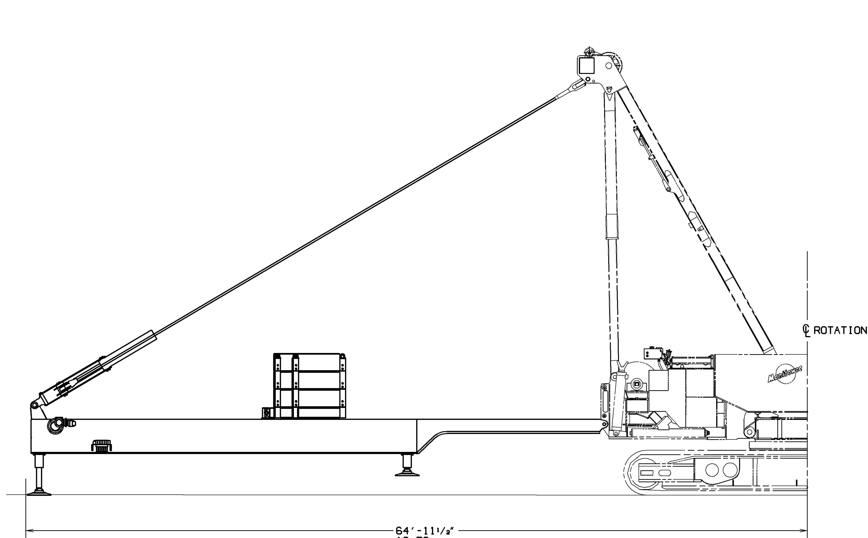
X-SPANDER
