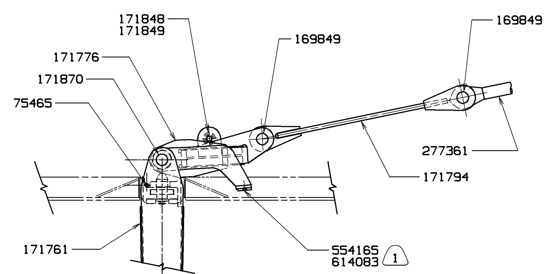
VIEW "G"
