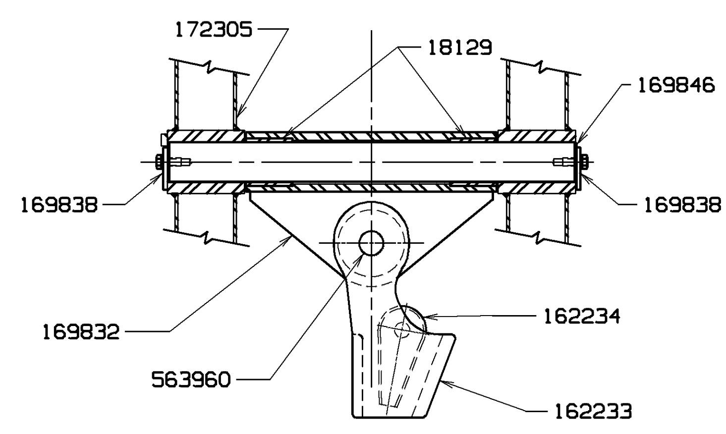
SECTION "D" - "D" SEE 7
