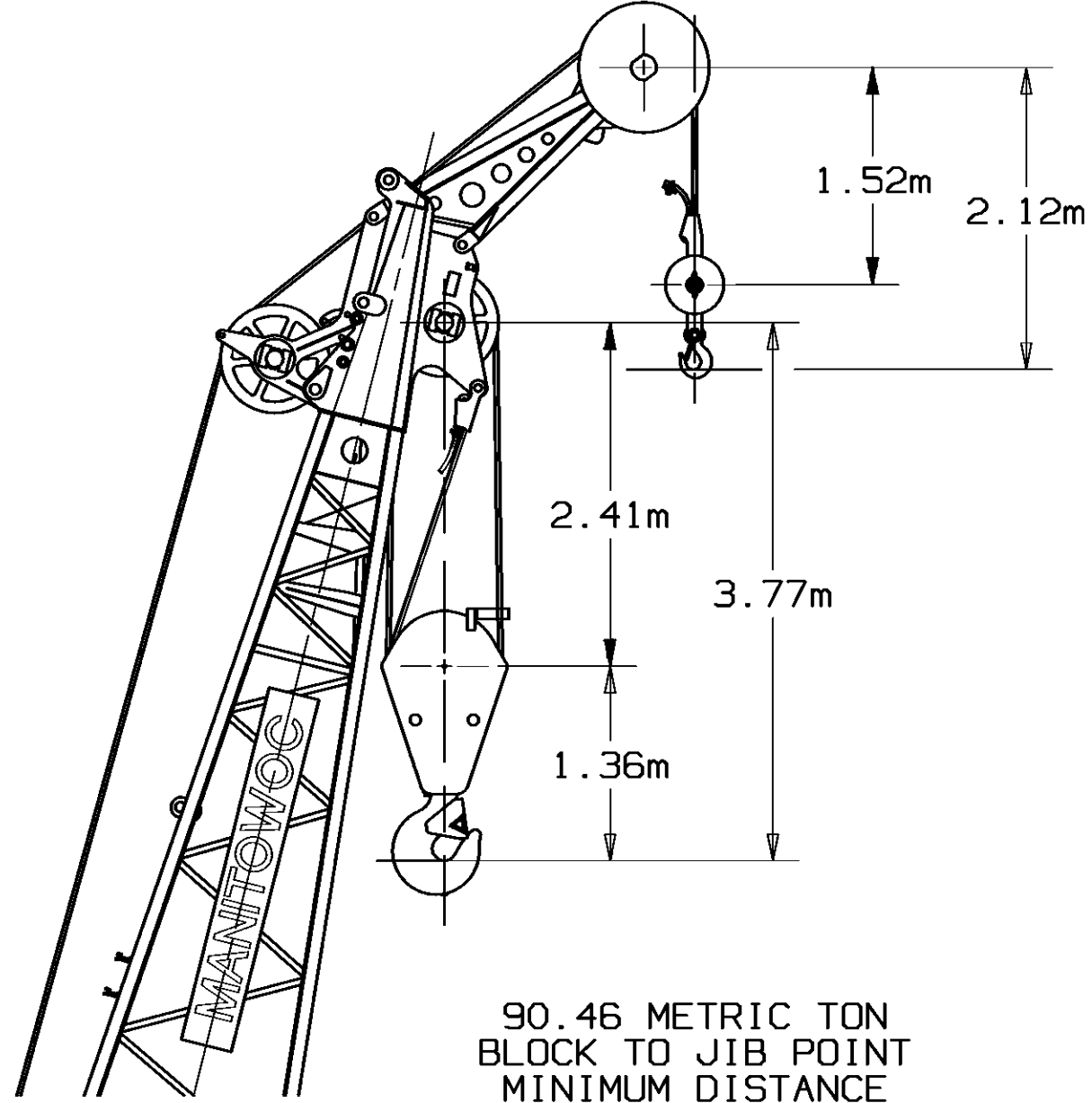
14 METRIC TON SWIVEL HOOK & WEIGHT BALL TO JIB POINT MINIMUM DISTANCE NO.149 JIB - SINGLE PART LINE
