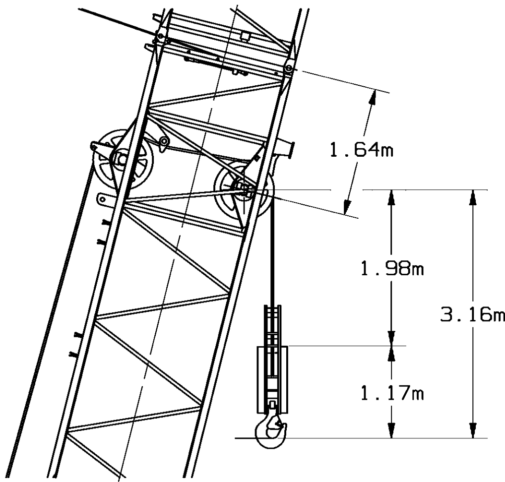
40.70 METRIC TON BLOCK TO INTERMEDIATE FALL MINIMUM DISTANCE NO.149 JIB - 2 PARTS OF LINE
