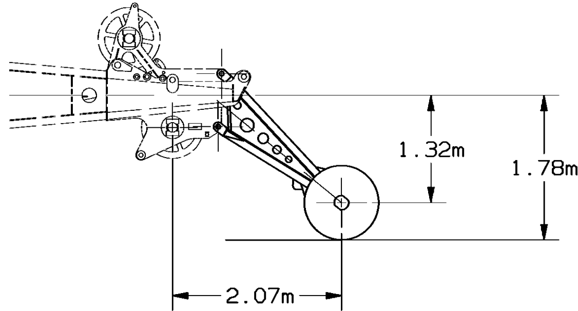
NO.149 JIB POINT ROLLER ASSEMBLY (SIDE VIEW)
